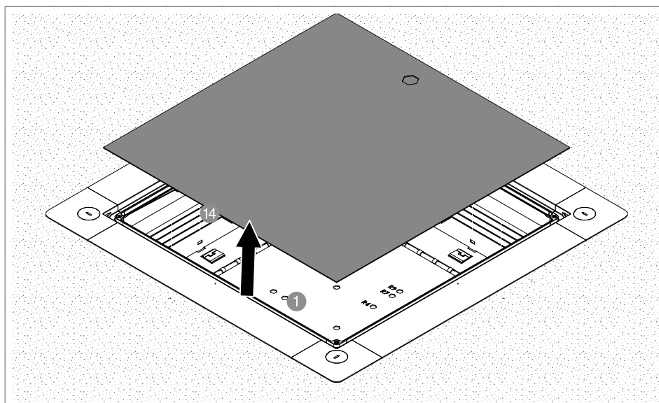
Fig. 49: Removing the mounting lid
