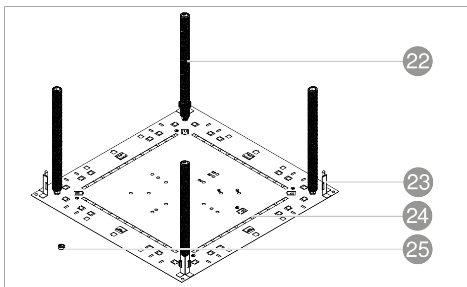
Fig. 6: System components – underfloor box base
