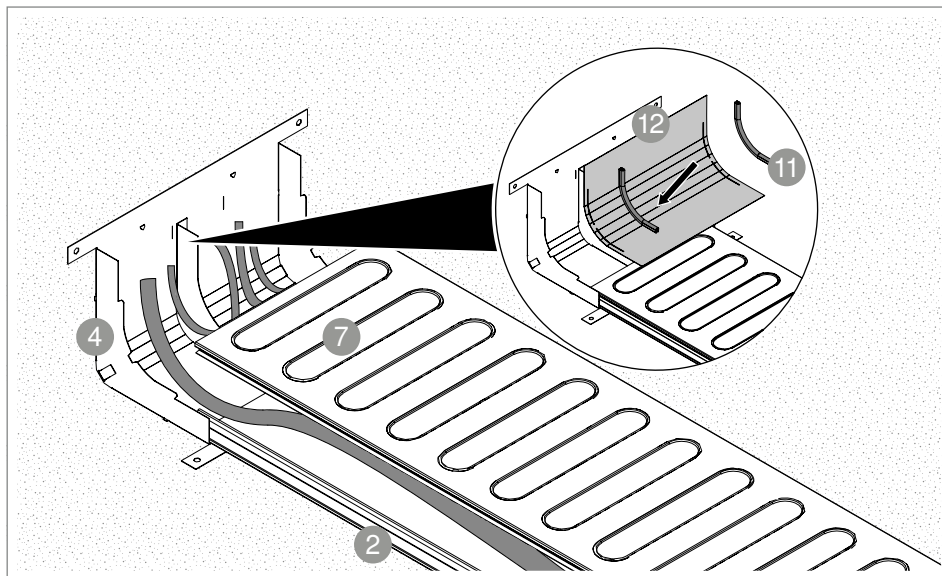
Fig. 25: Closing off the vertical bend
