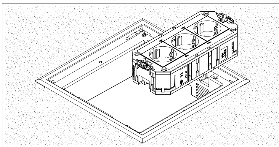
Fig. 58: Performing the electrical installation
