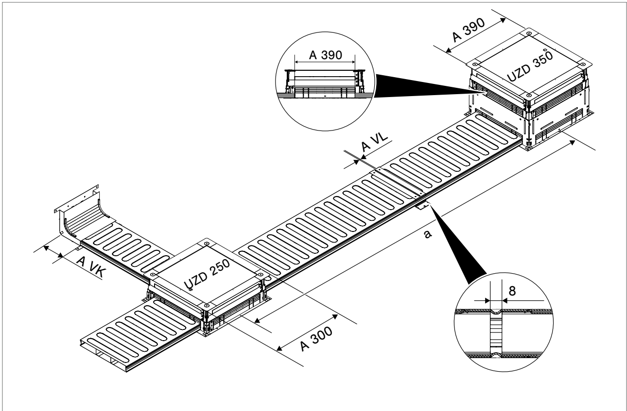
Fig. 9: Deduction dimensions
