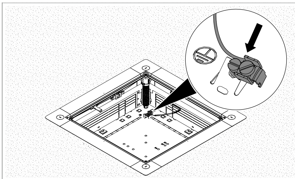
Fig. 53: Creating the earthing connection
