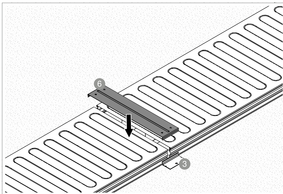
Fig. 26: Locking on the connection shackle cover
